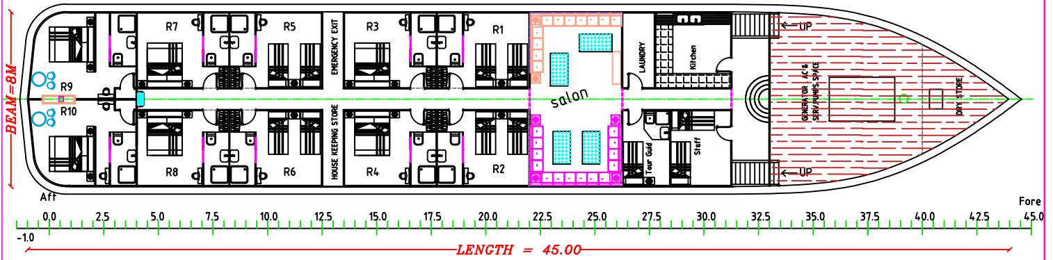
CABINS DISTRIBUTION PLAN
